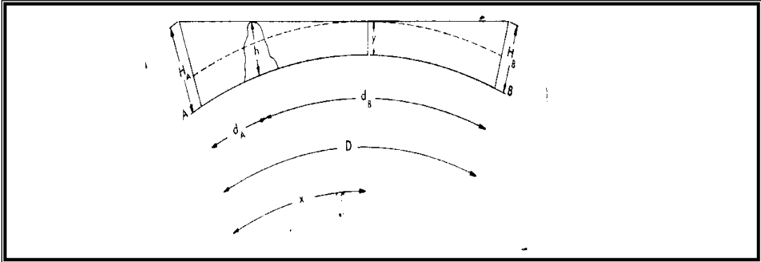
Fig. 2.14 “Intervisibility of Geodetic Station”
