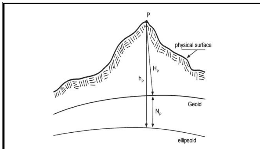
Fig. 2.5 "Vertical Datum"
