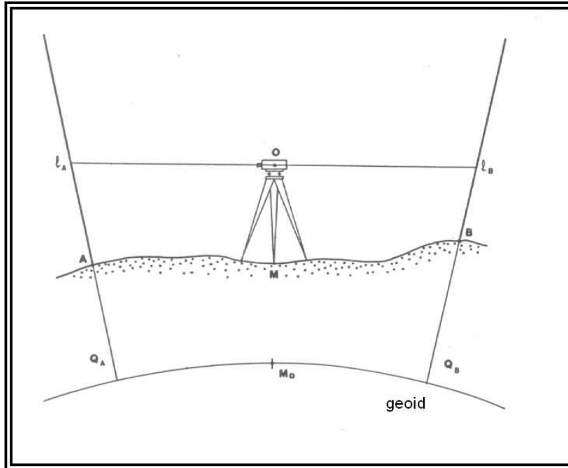
Fig. 2.15 “Geometric levelling”
