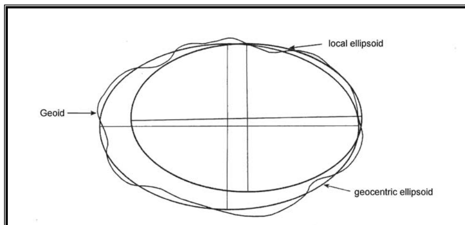
Fig. 2.3 "Datum orientation"
