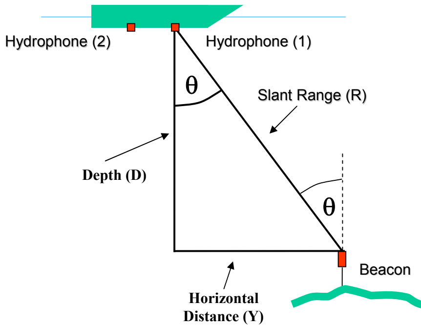
Fig. 2.25 “Range determination”
