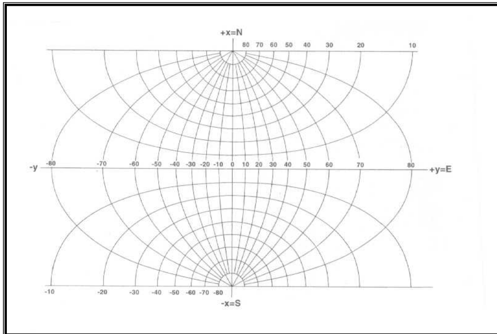
Fig. 2.6 “Geographic grid”
