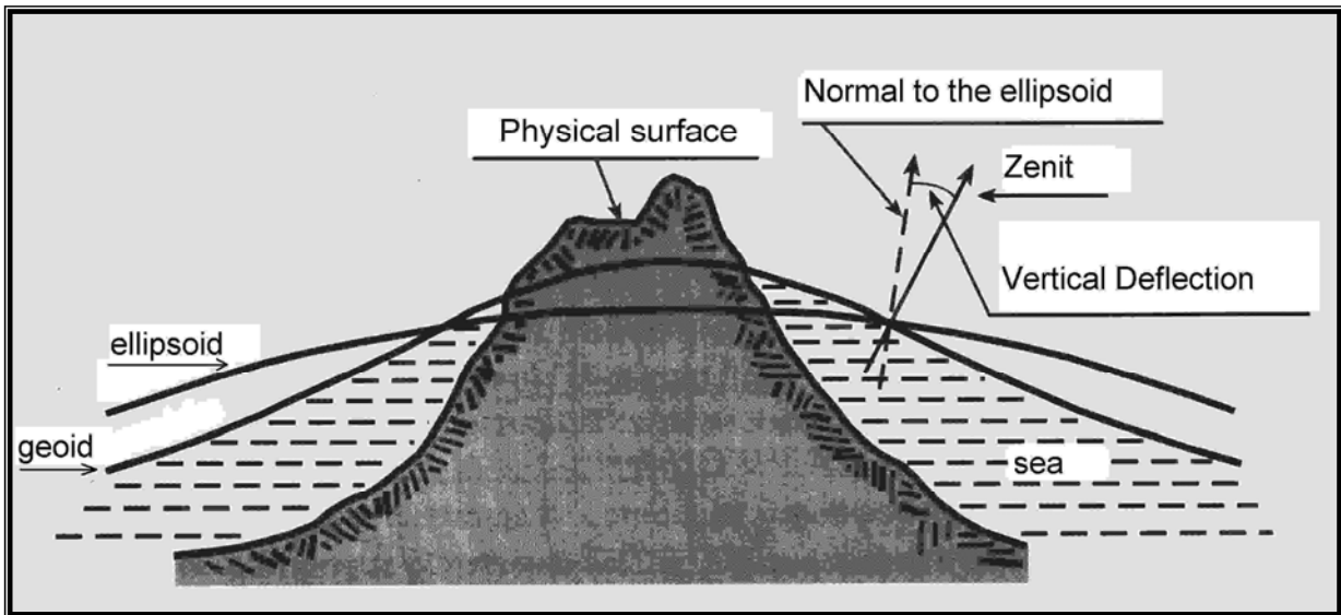
Fig. 2.1 "The Earth"
