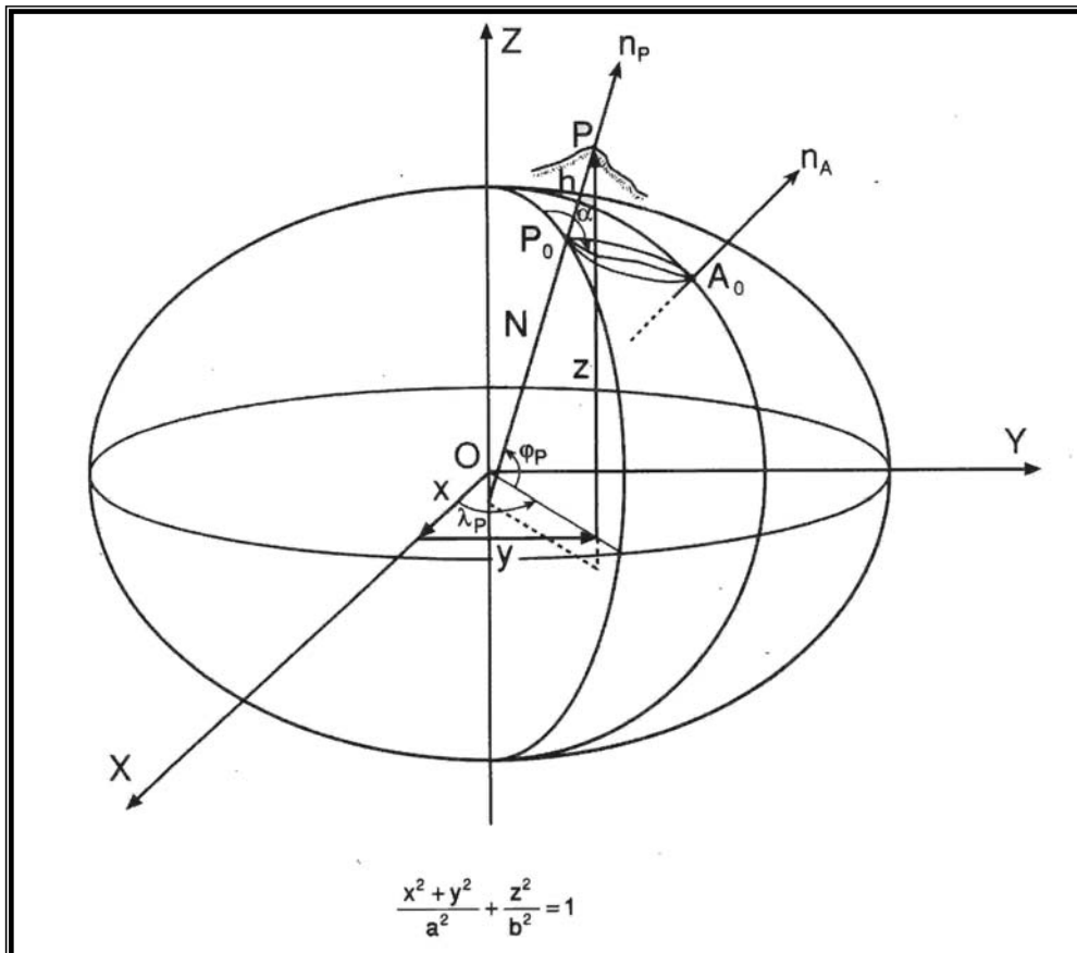
Fig. 2.2 "The Ellipsoid"
