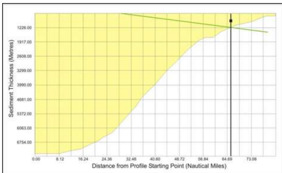
Figure 5.7 – This illustrates the determination of the point where the thickness of sedimentary rocks is equal to 1% of the distance back to the foot of the continental slope. The coloured portion of the plot represents a profile of sediment thickness (the top 500 metres or so are not
