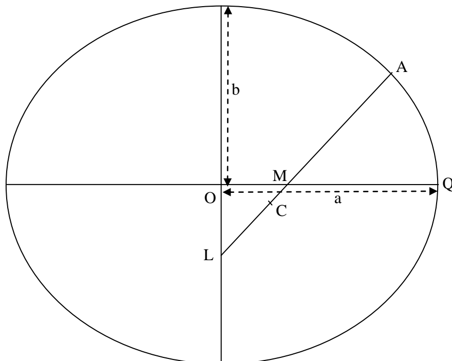
Figure 3.10 – Cross-section through an Ellipsoid to illustrate polar flattening The effect is greatly exaggerated in the diagram. In fact the flattening is not great, and the polar
