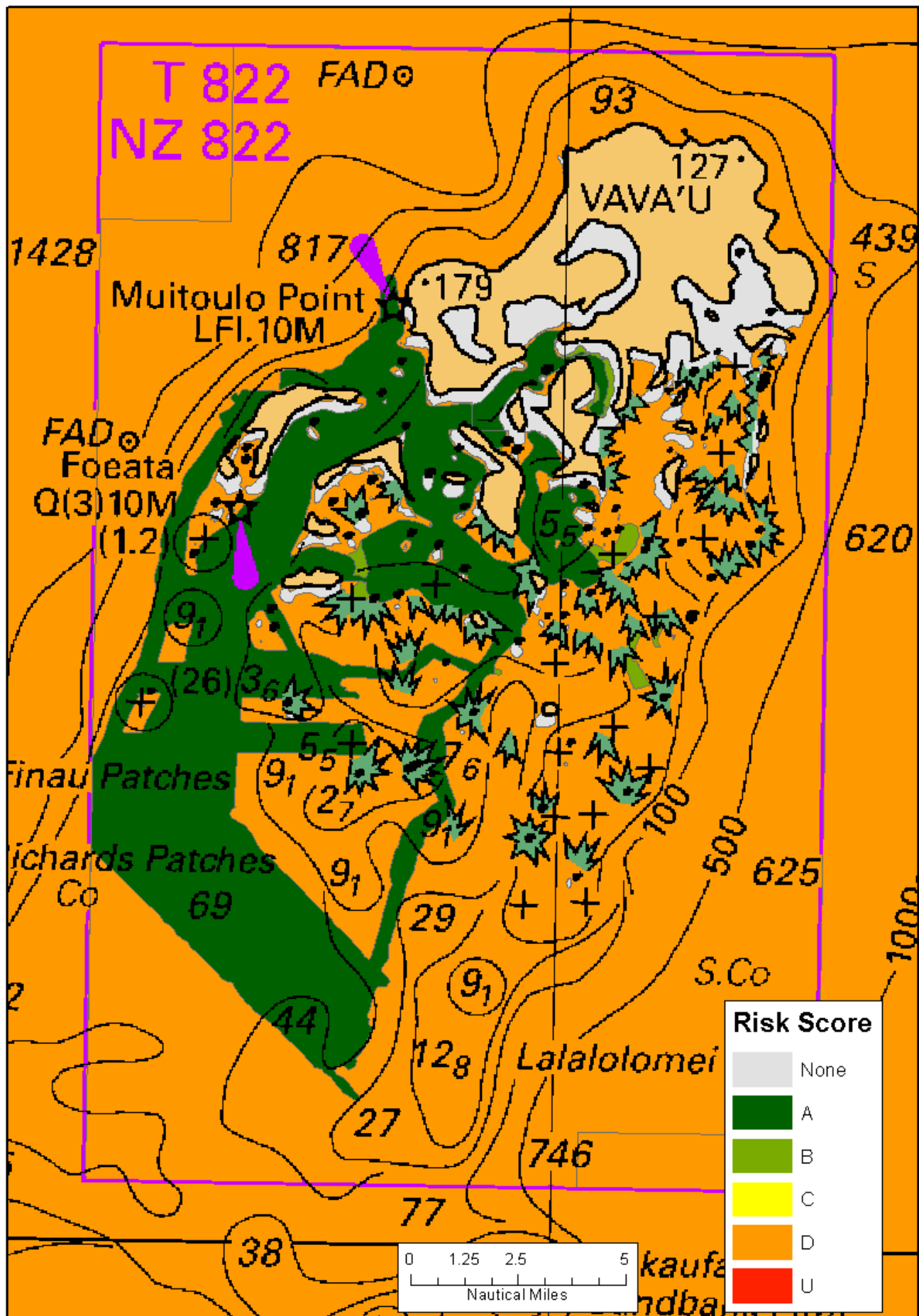
Figure 34: CATZOC Categories for Vava'u Island Group
