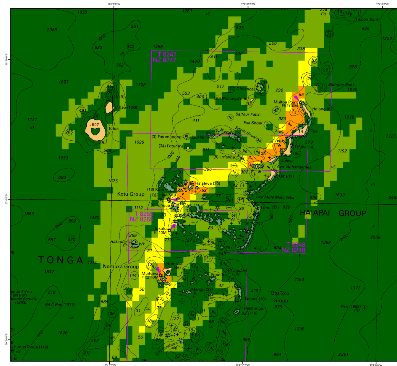
Figure 56 : Traffic Forecast Risk Result for Ha'apai
