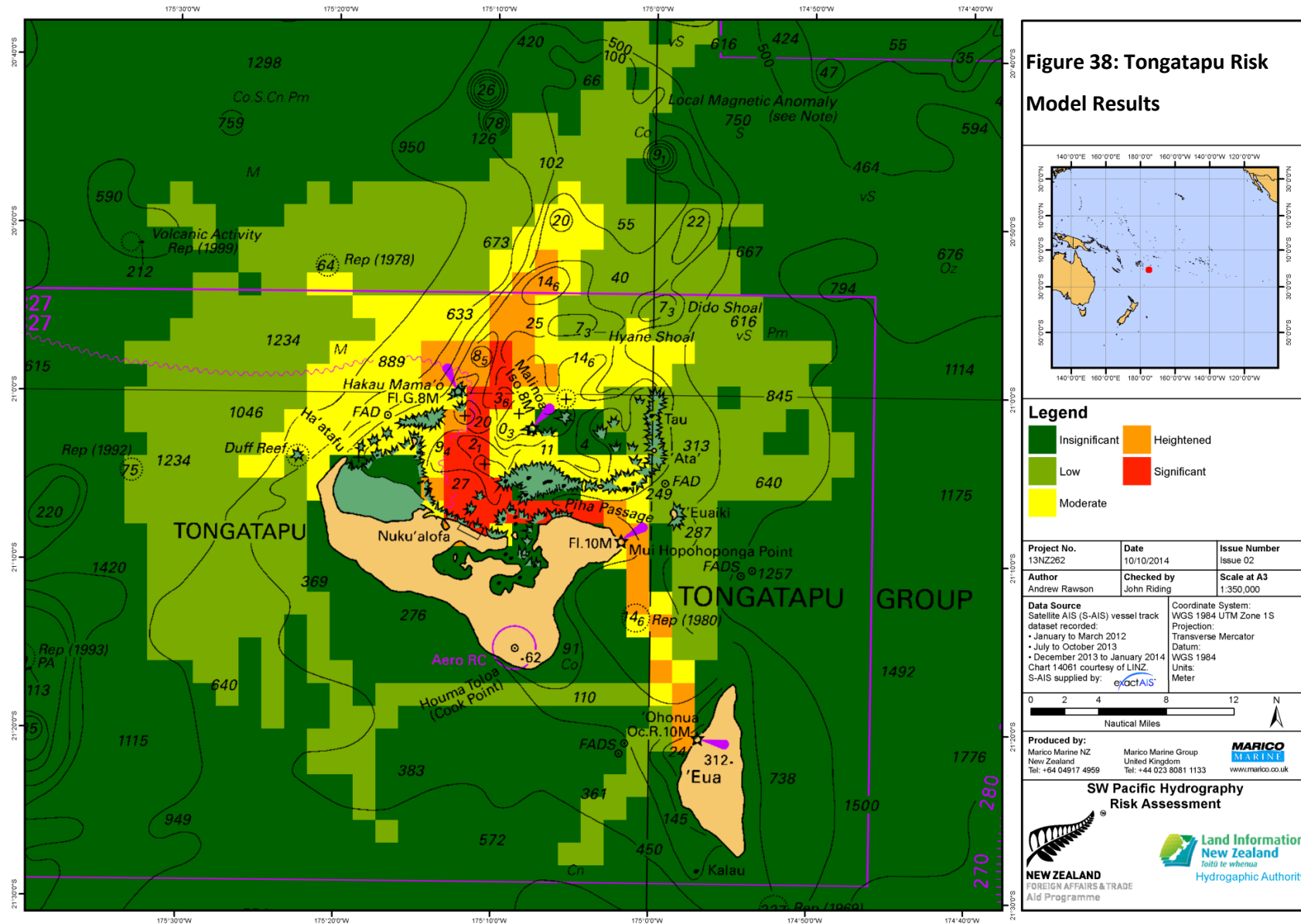
Figure Reference: 13NZ262_Tonga_RiskModel7_02
