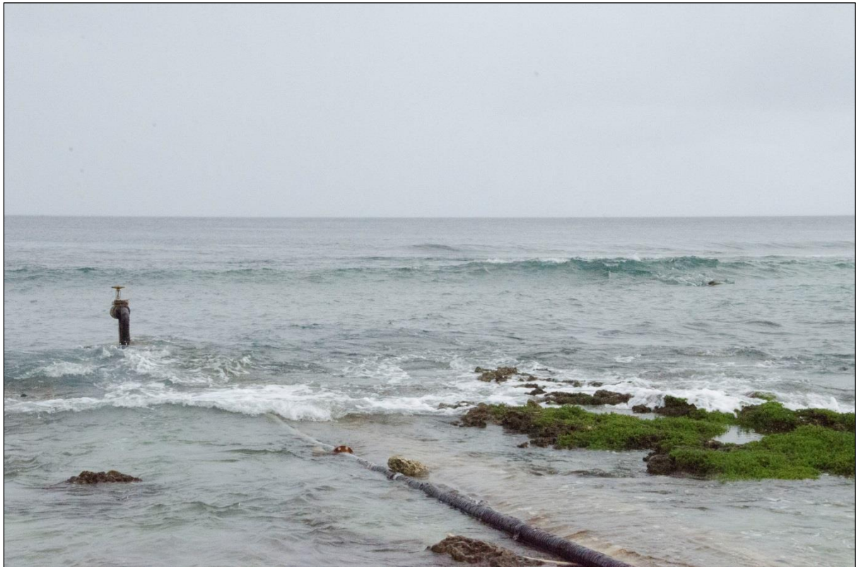
Figure 6 : The Coastal Fuel Manifold Installed in the Surf at 'Eua
