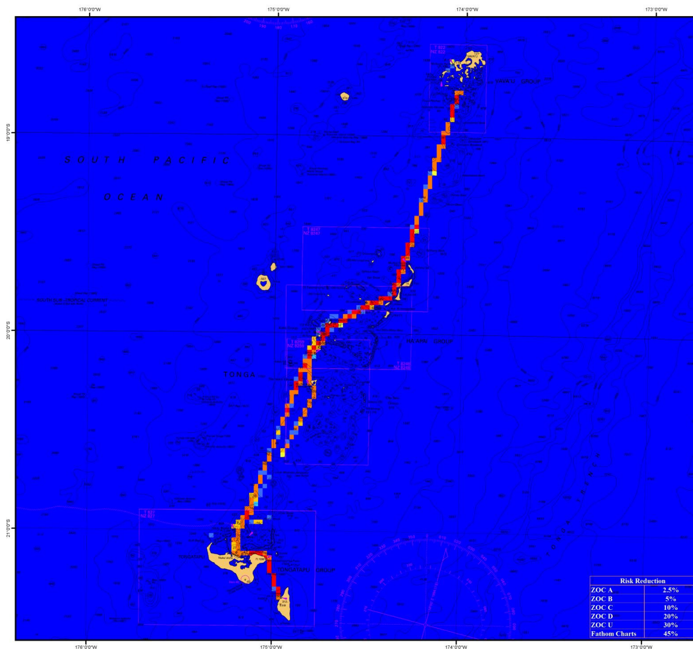
Figure 51: Cost Benefits Results for Tonga – Costed as Singlebeam Survey ($500)
