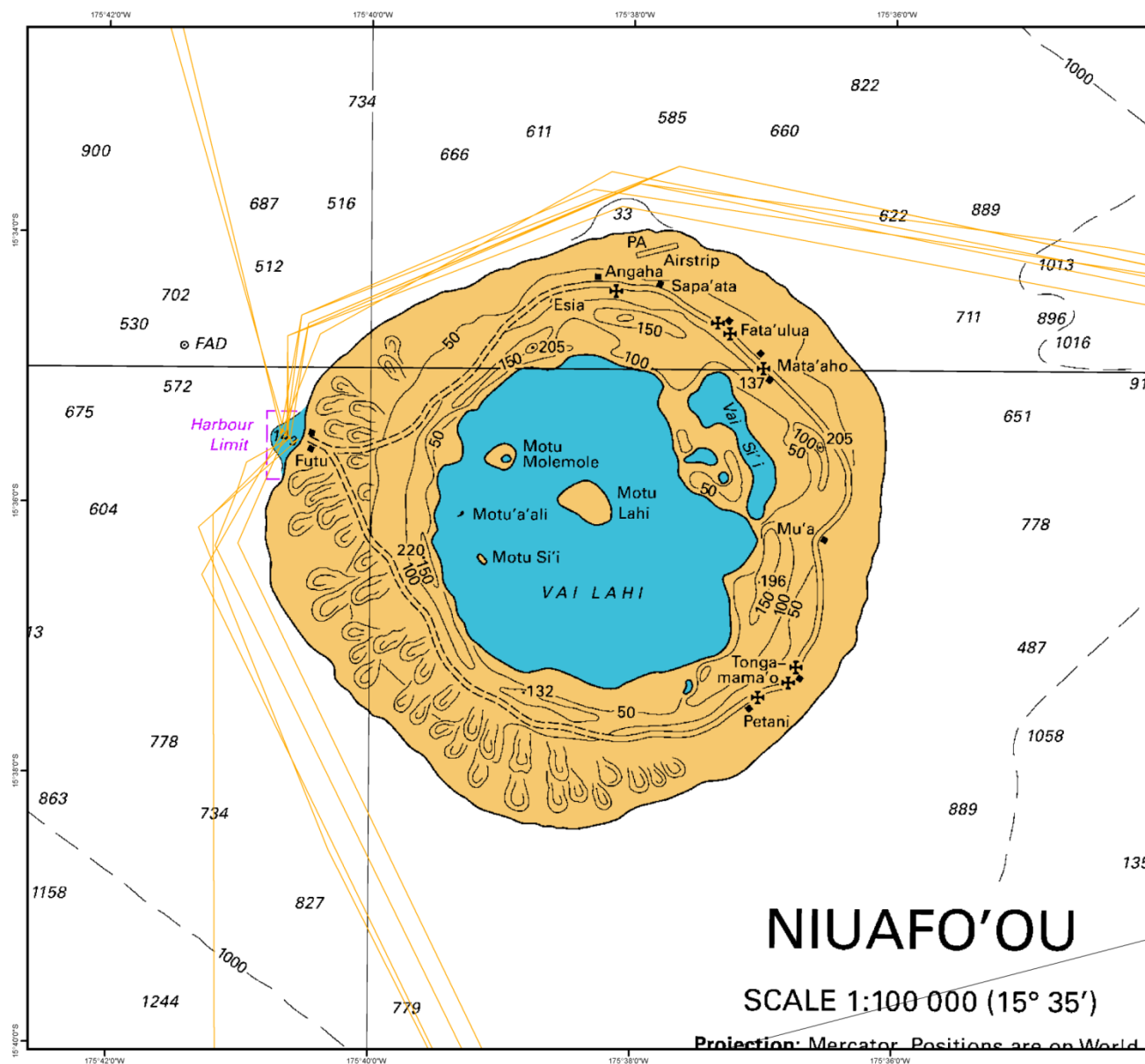
Figure 30: Niuafu'ou Island Vessel Tracks
