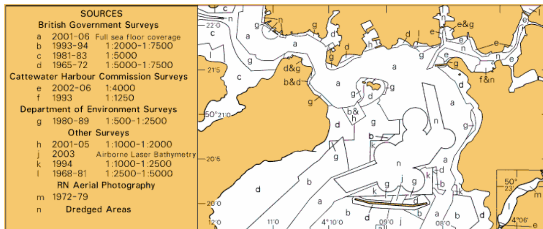
Figure 2.3.1 Source Diagram
