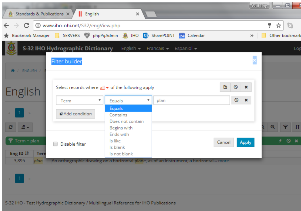
Filter builder
