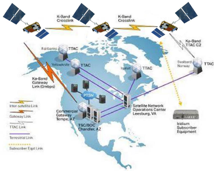
Figure 7— The Iridium global satellite system, network overview (North and Central America)
