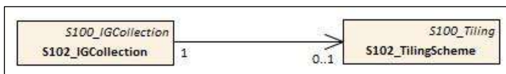
Figure 4.6 - Feature Association
