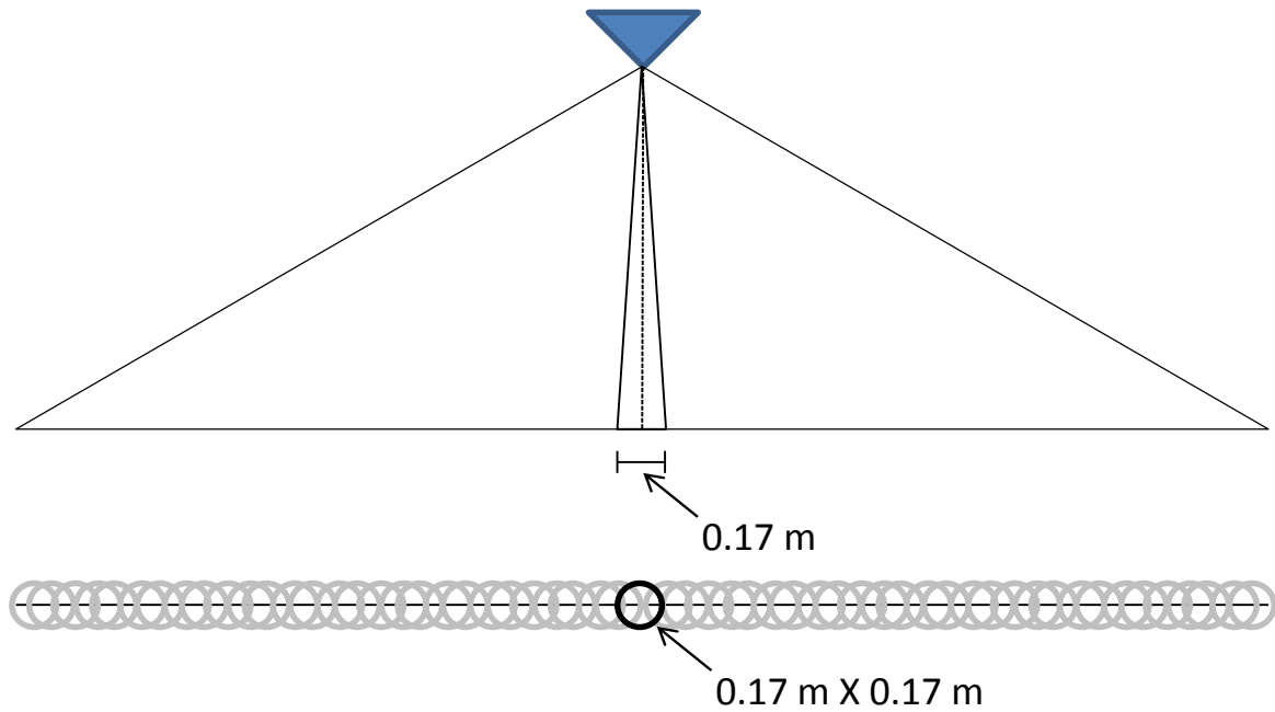
Figure I.1 - Sonar Footprint at Nadir
