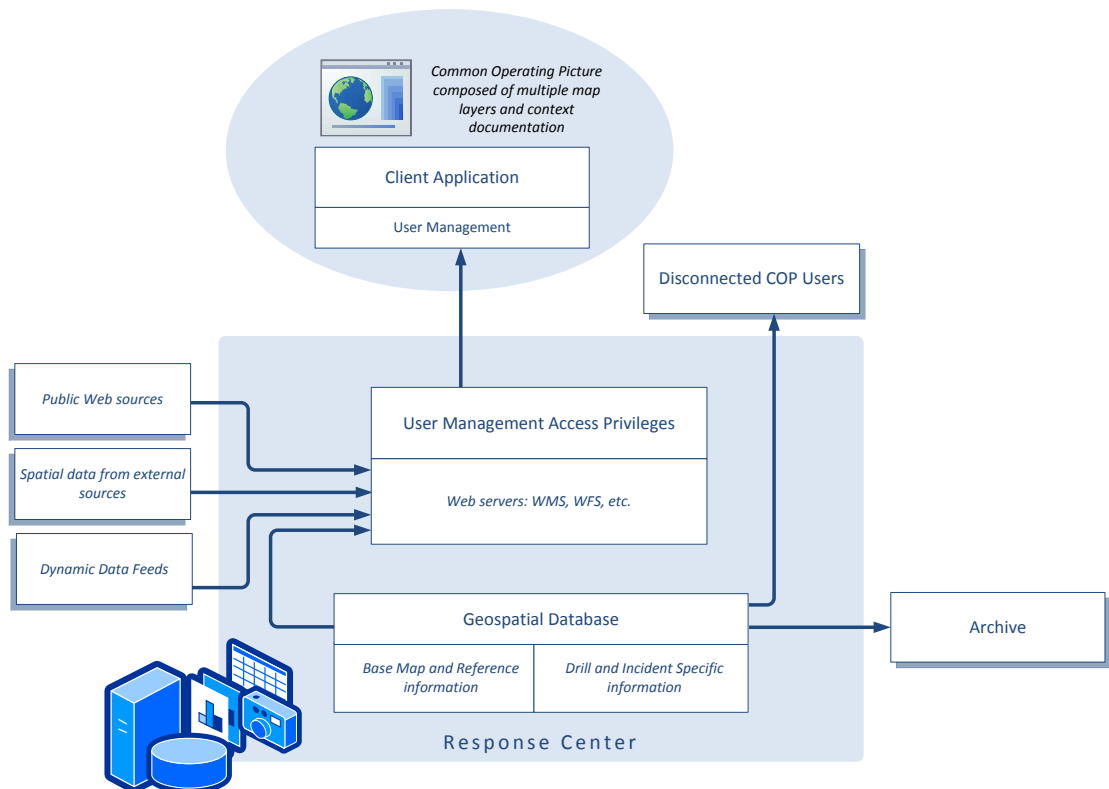
Figure 16 COP service-oriented architecture
