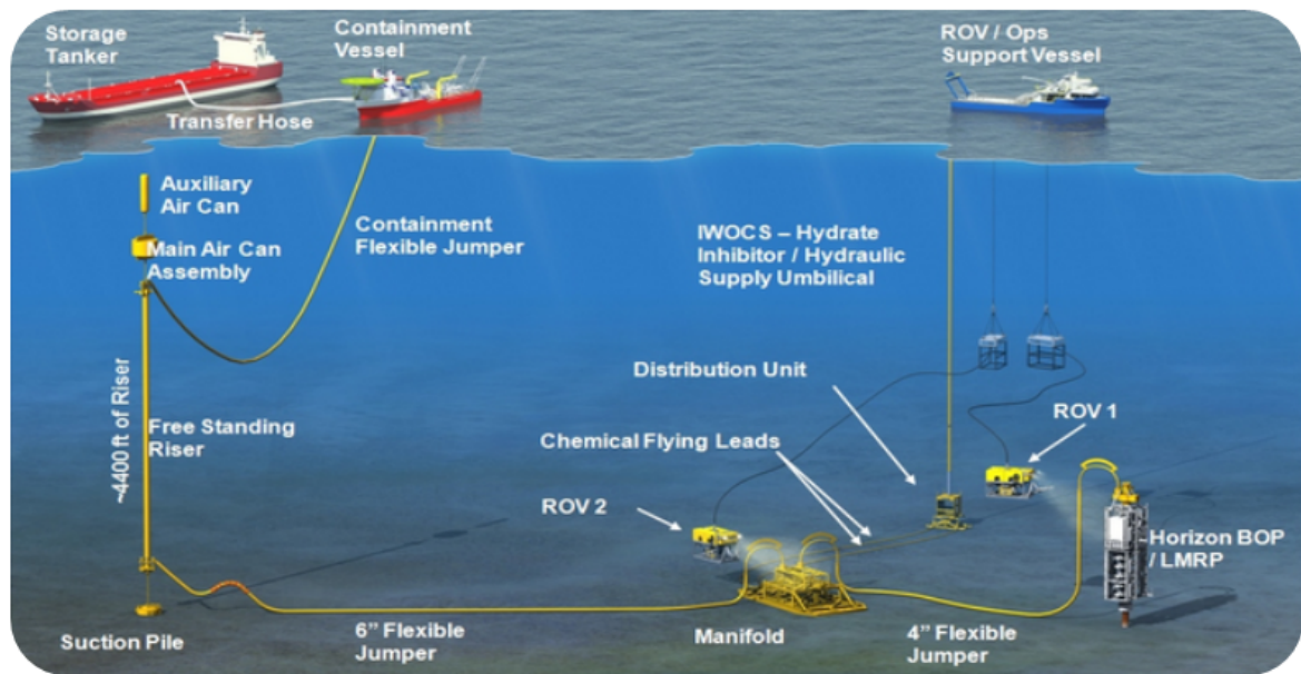
Figure 1 Typical subsea well intervention project
