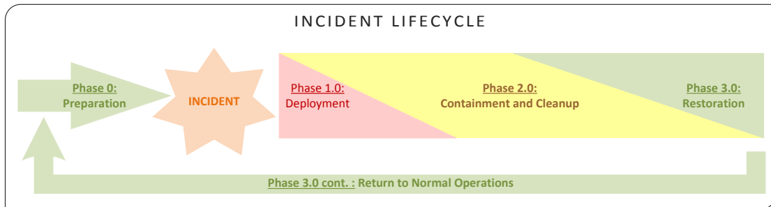
Figure 4 Incident lifecycle
