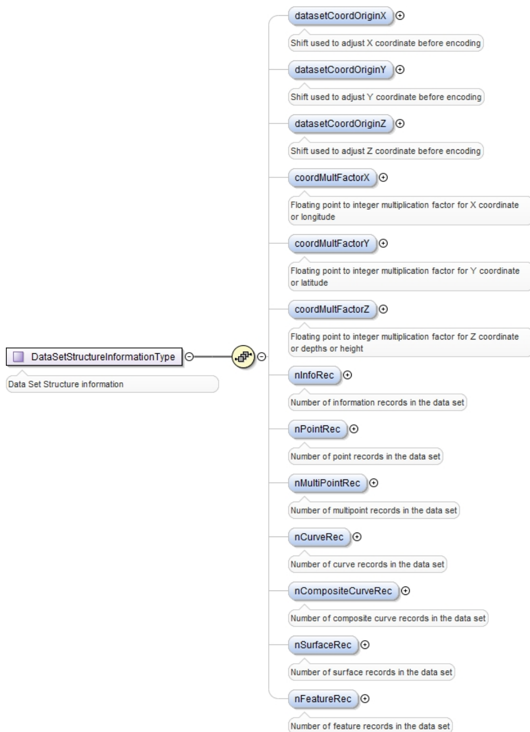
Figure 10b-13 – Dataset structure information
