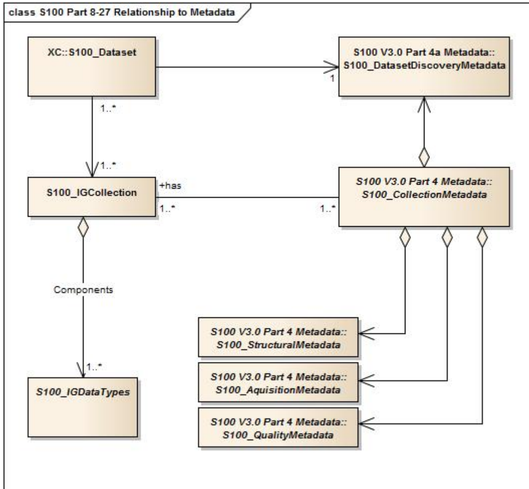
ure 8-27 – Relationship to Metadata
