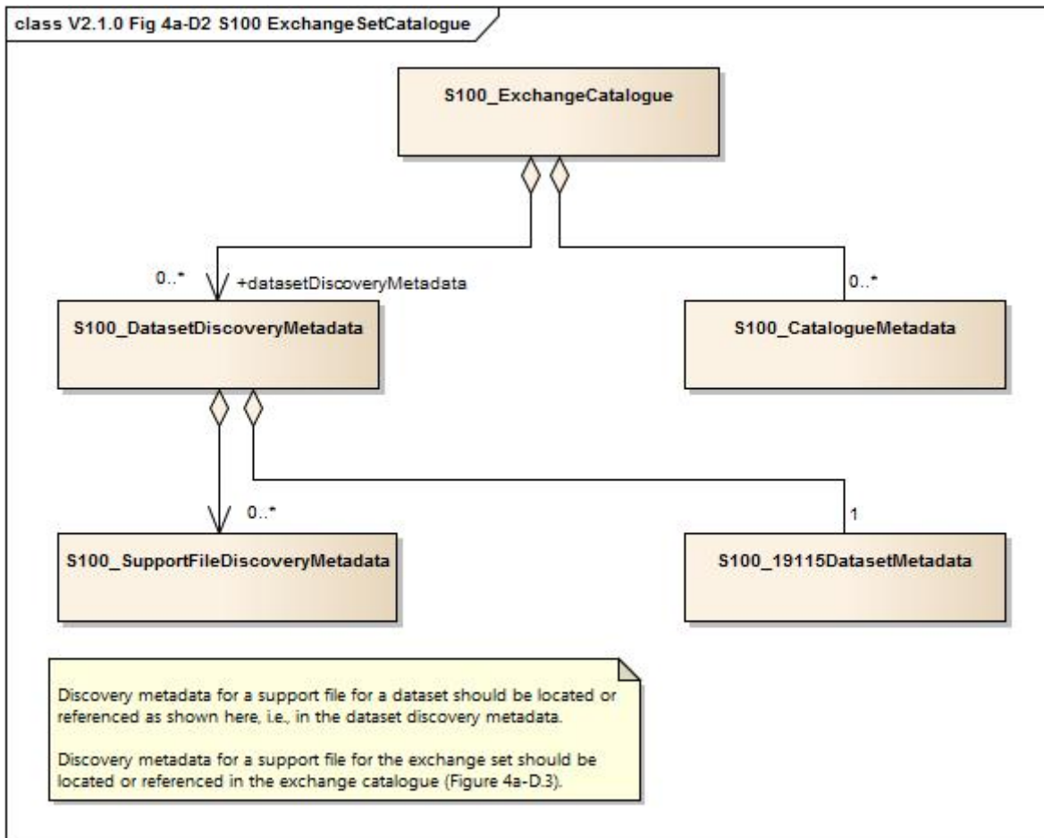
Figure 4a-D-2 – S-100 Exchange Set Catalogue
