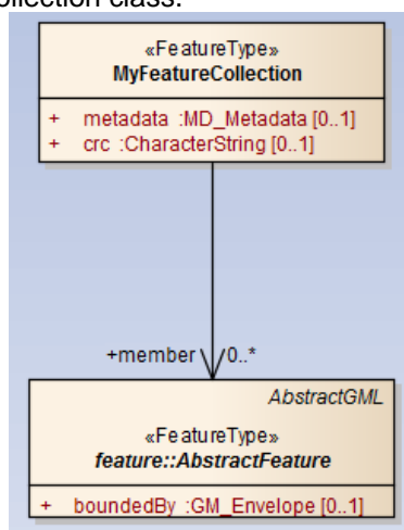
Figure 10b-15 – Encoding dataset metadata and integrity check properties
