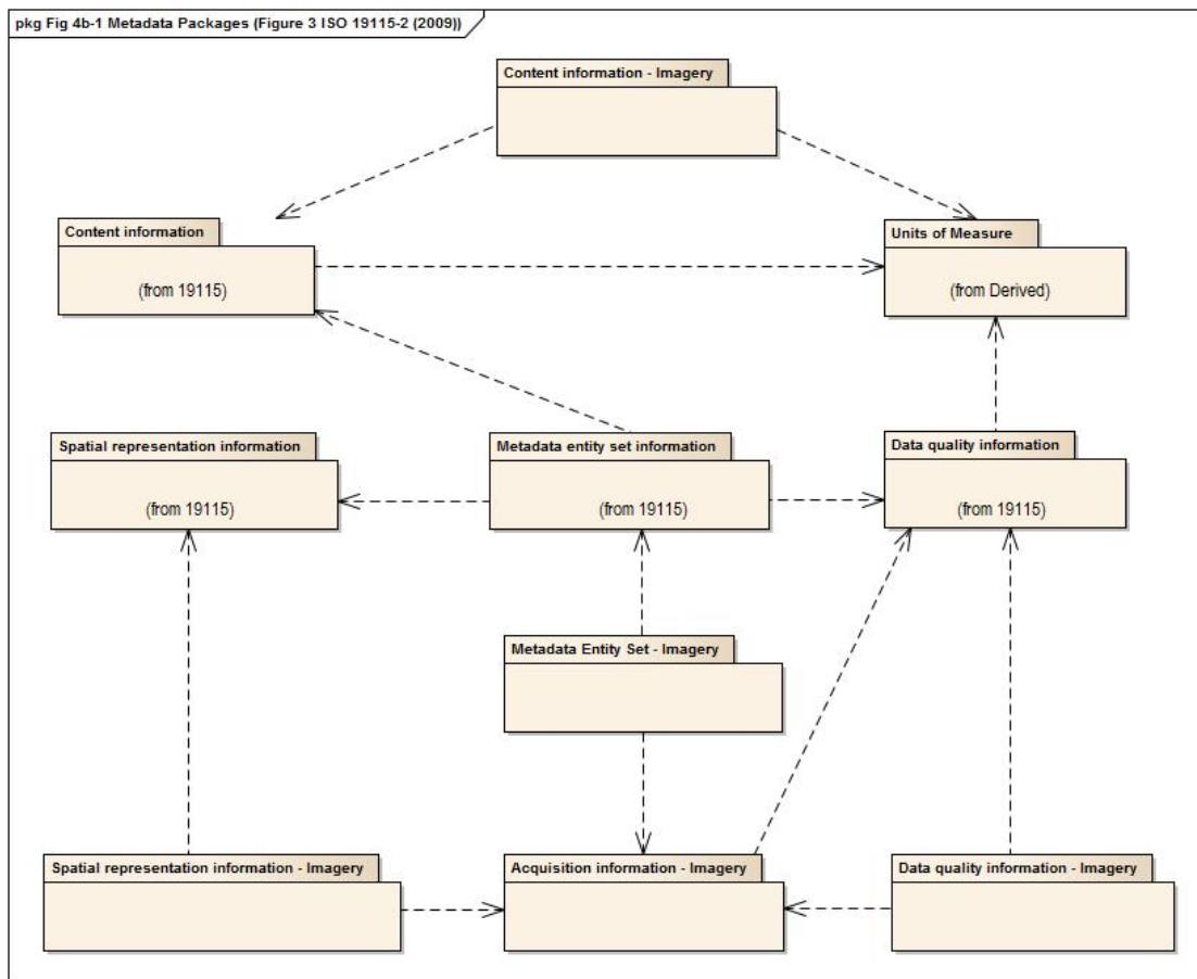
Figure 4b-1 — Metadata packages
