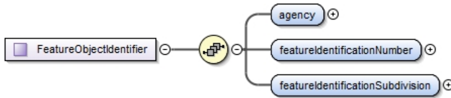
Figure 10b-14 – Structure of feature object identifier element
