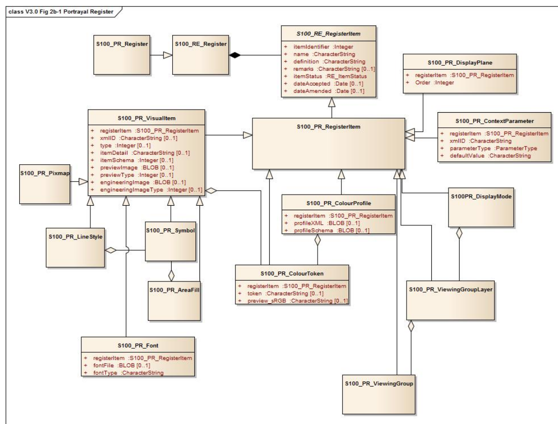
Figure 2b-1 – Portrayal Register
