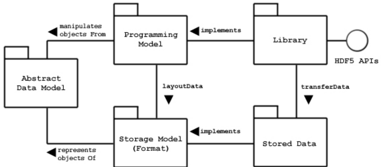
Figure 1 - Abstract Data Model
