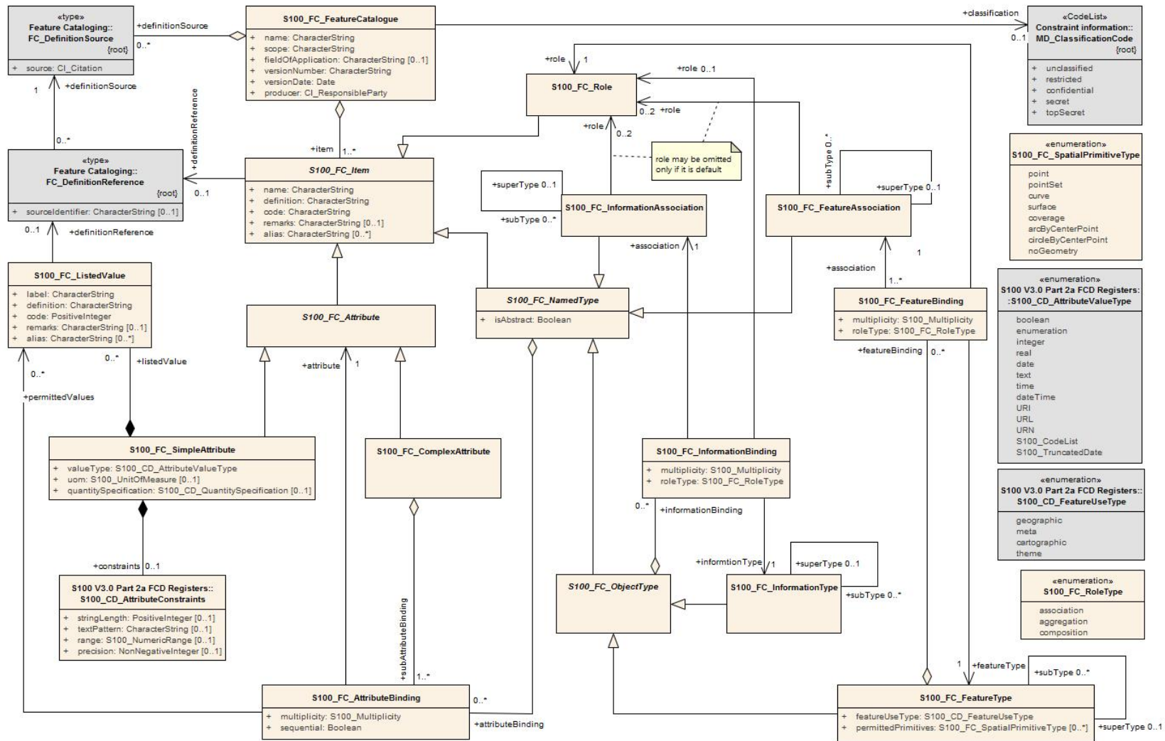
Figure 5-A-1. Feature Catalogue — UML Model
