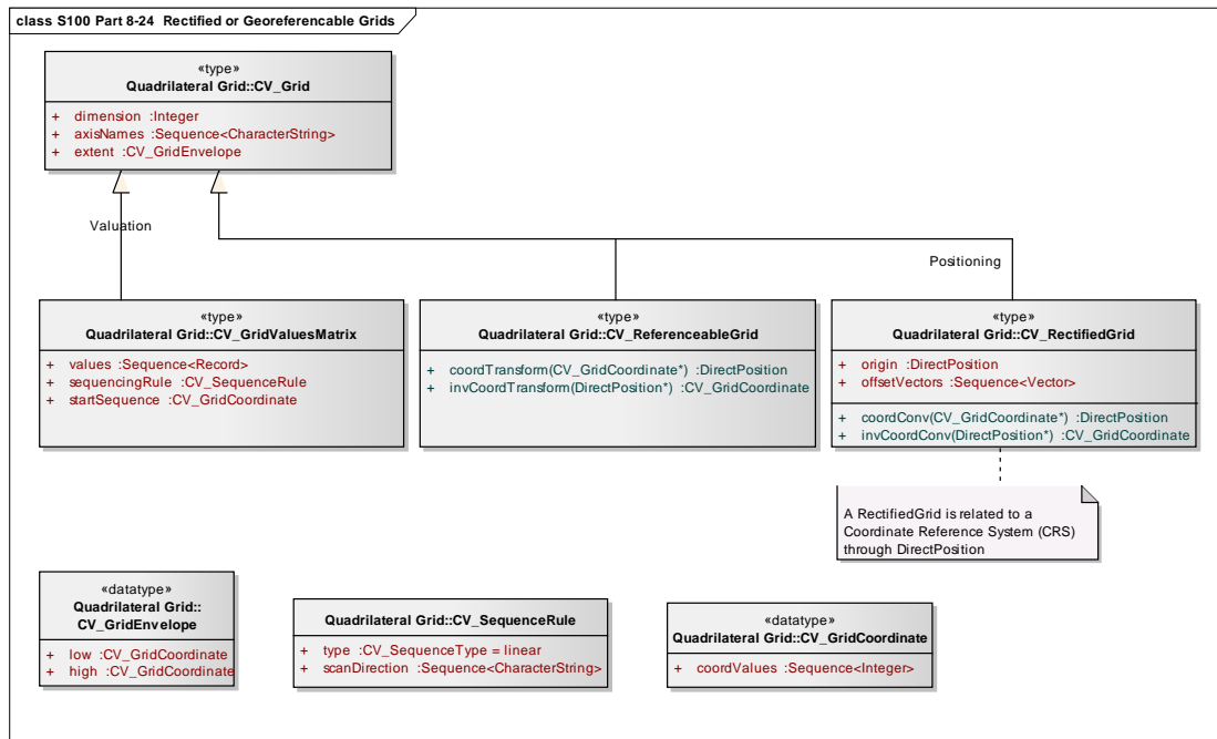
Figure 8-24 - Rectified or Georeferencable Grids
