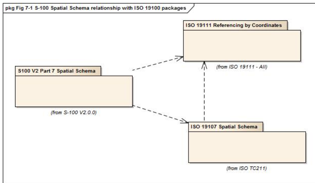
Figure 7-1 — S-100 Spatial Schema relationship with ISO 19100 Packages
