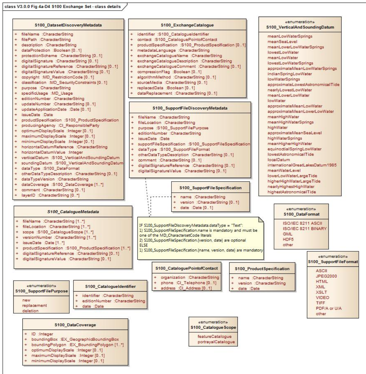
Figure 4a-D-4 S-100 Exchange Set - class details
