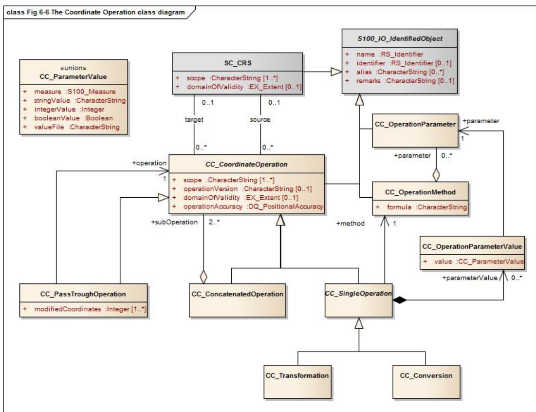
6-4.6 The Coordinate Operation package
