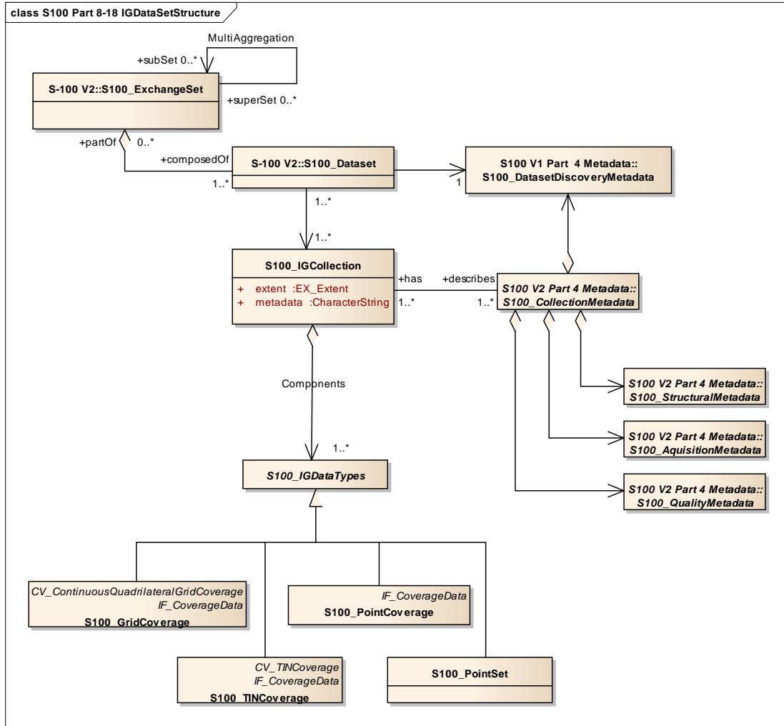
Figure 8-18 – Data Set Structure
