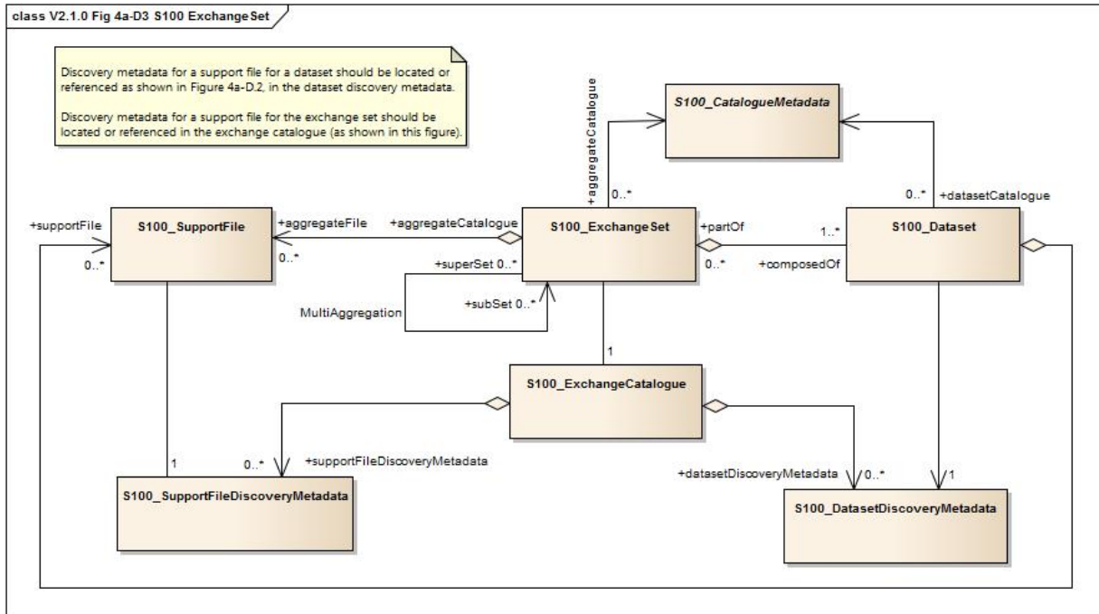
Figure 4a-D-3 – S-100 Exchange Set
