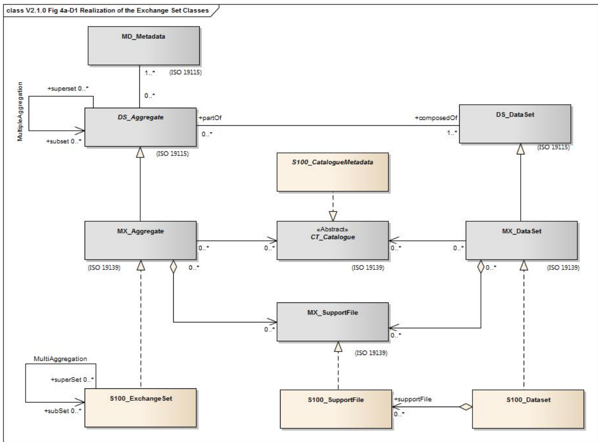
Figure 4a-D-1 Realization of the Exchange Set Classes
