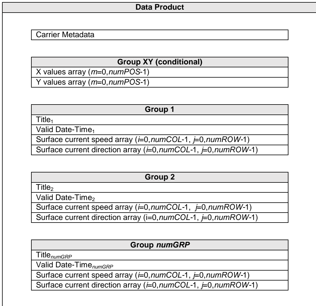
Figure 0.1 - Schematic of the S-111 data product structure. The four parameters numPOS , numCOL , numROW , and numGRP are explained in Table 10.2. Group XY appears only for dataCodingFormat = 1, 3 or 4 (Table 10.1).
