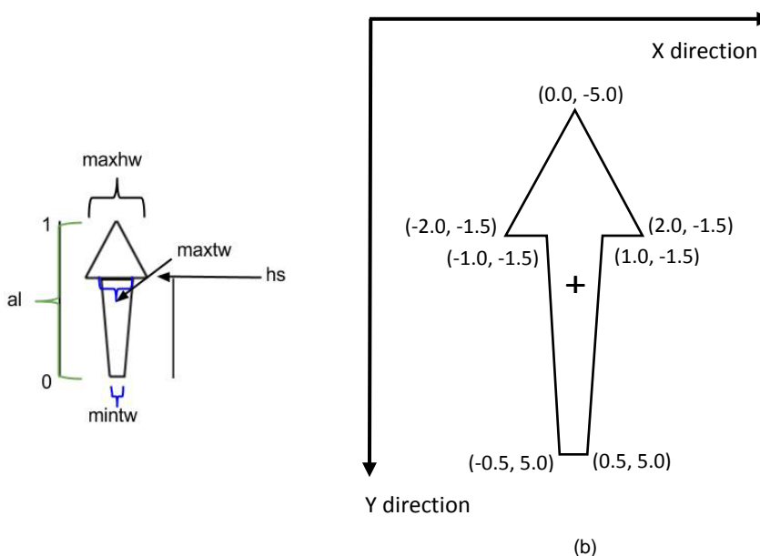
Figure 9.1 – (a) Generalized arrow shape for use in representing surface currents. (b) The arrow with vertex coordinates (x, y) in mm. The '+' shows the location of the pivot point at (0.0, 0.0) and the y axis is pointing downward.
