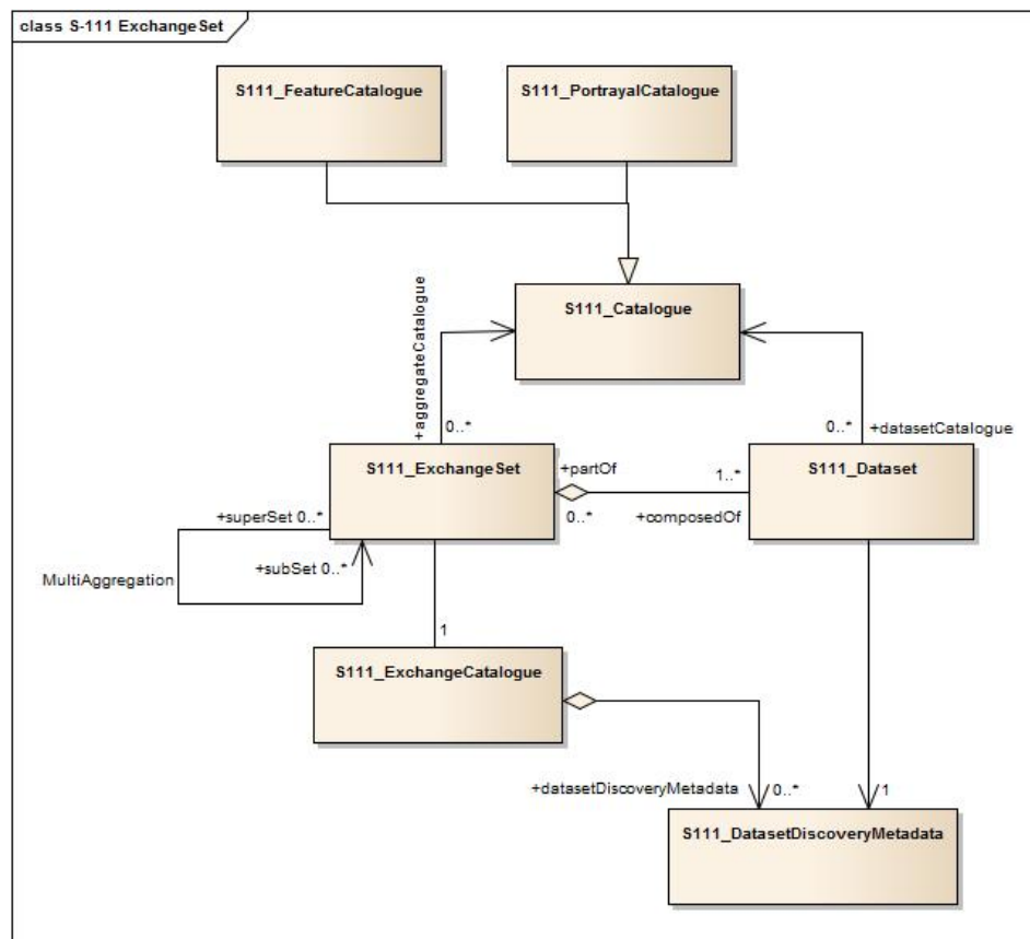
Figure 12.3 – S-111 ExchangeSet.
