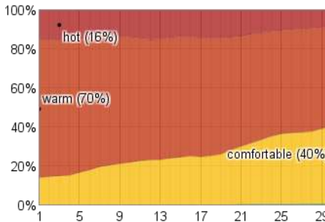
The average fraction of time spent in various temperature bands: frigid (below -9°C), freezing (-9°C to 0°C), cold (0°C to 10°C), cool (10°C to 18°C), comfortable (18°C to 24°C), warm (24°C to 29°C), hot (29°C to 38°C) and sweltering (above 38°C).
