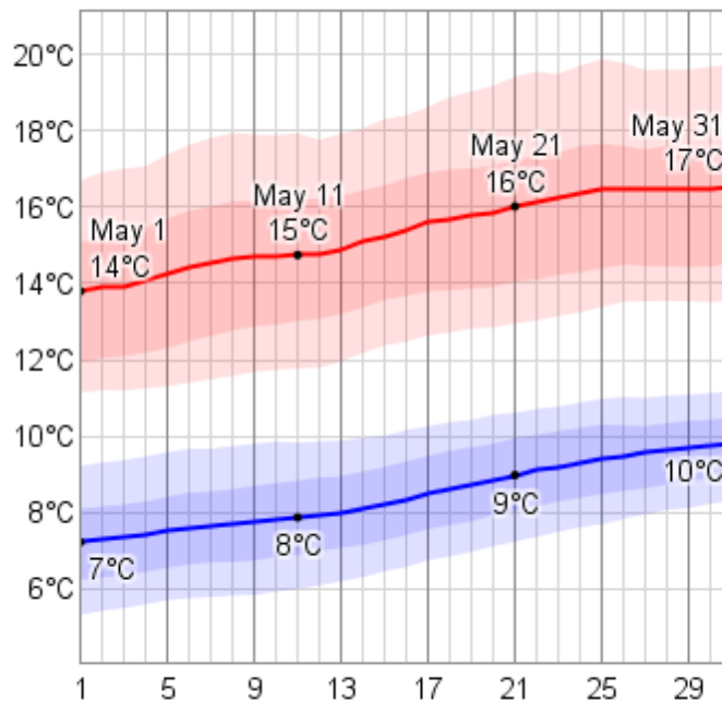
The daily average low (blue) and high (red) temperature with percentile bands (inner band from 25th to 75th percentile, outer band from 10th to 90th percentile).
