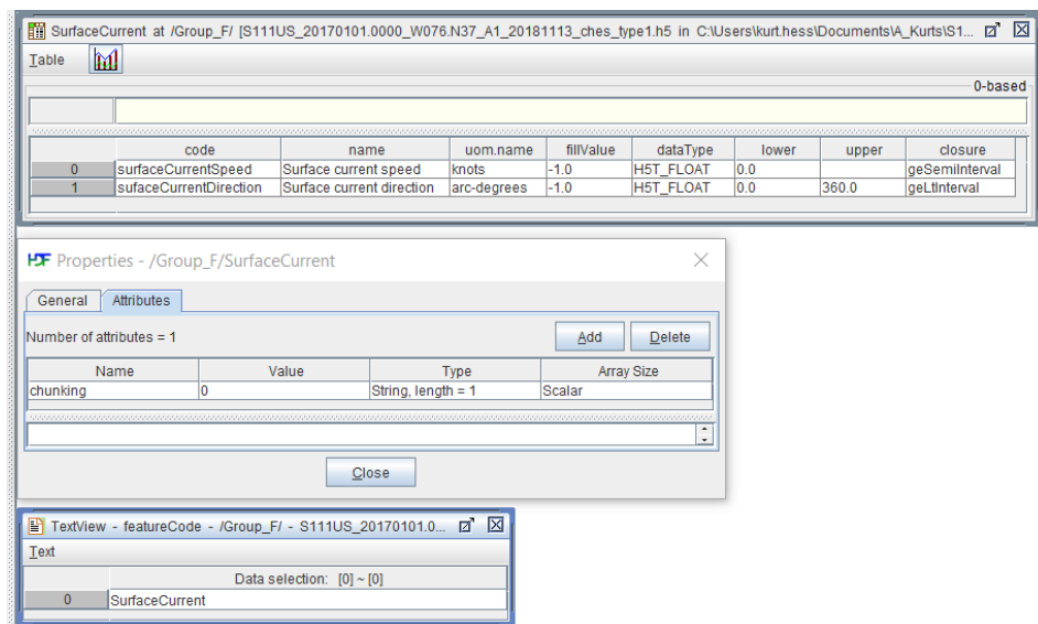
Figure F.1 - Typical HDF5 file and its two groups, 'Group_F' and 'SurfaceCurrent'
