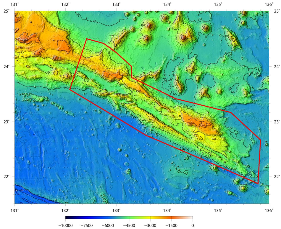
Fig 1. Color shaded bathymetric map of the Oki-Daito Ridge. Contours are in 200 m. The polygon delineating the feature is shown in red line.
