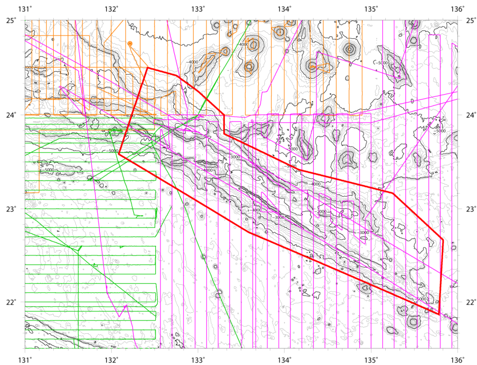
Fig 2. Bathymetric map of the Oki-Daito Ridge. Contours are in 200 m. The polygon delineating the feature is shown in red line. The ship track are shown in green (for surveys in 1996 and 1997), orange (for surveys in 2001), and purple (for surveys in 2005) lines.
