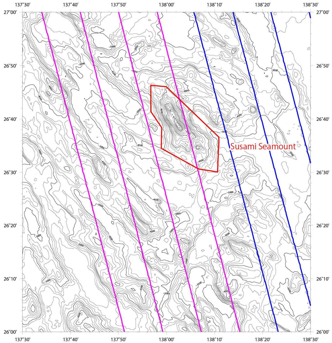
Fig 2. Bathymetric map of the Susami Seamount. Contours are in 100 m. The polygon delineating the feature is shown in red line. The ship track are shown in blue (for surveys in 2002) and purple (for surveys in 2003) lines.
