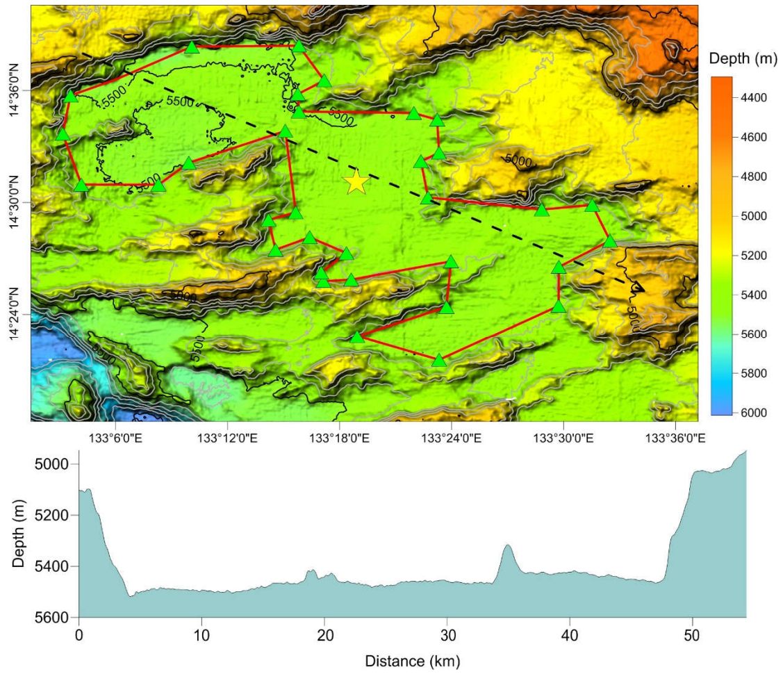
Fig.5 Bathymetric map and profile of Xiaoshu Basin
