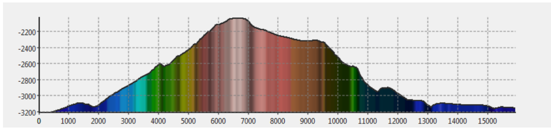
Fig.5. Profiles bathymetric map of ZiyouHill
