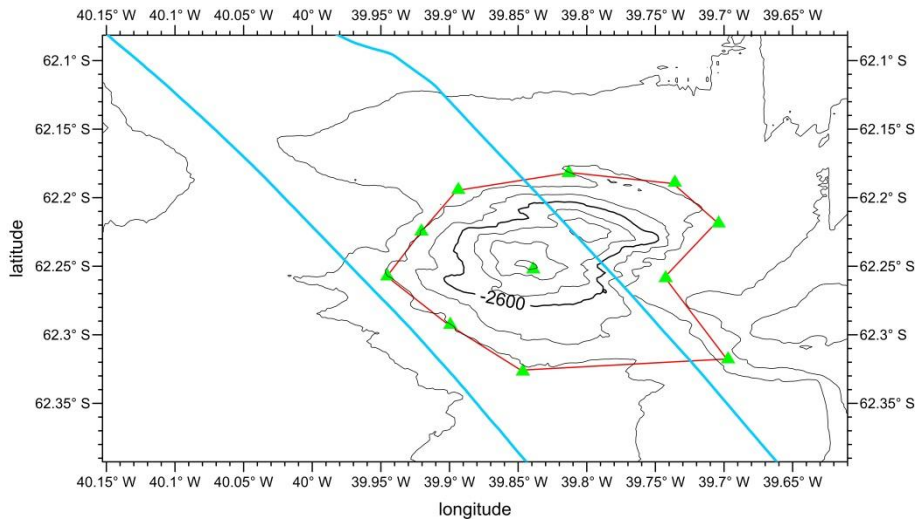
Fig.3. Bathymetric map of Ziyou Hill, showing track lines. Contours are in 200m
