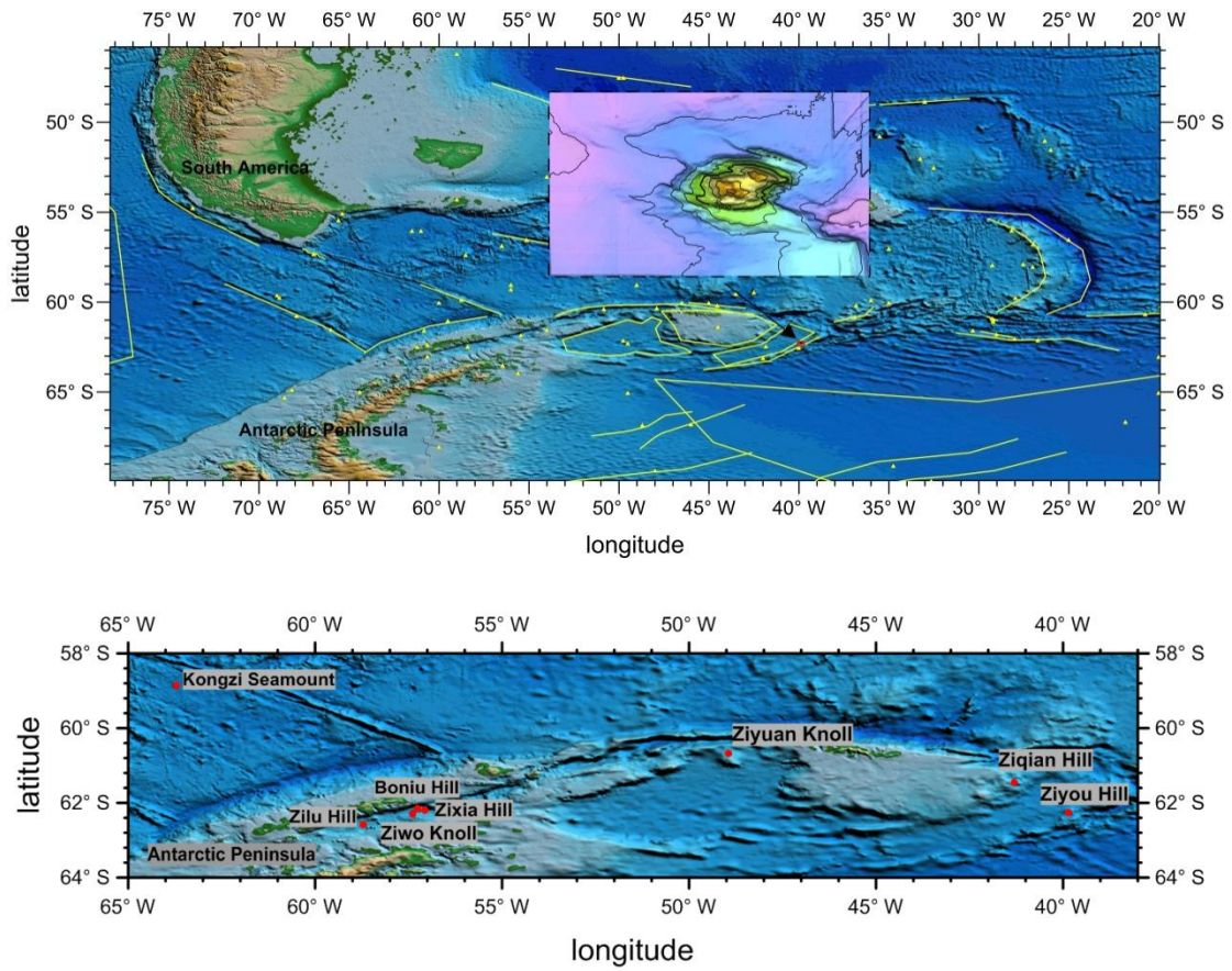
Fig.1. Index map showing the location of Ziyou Hill
