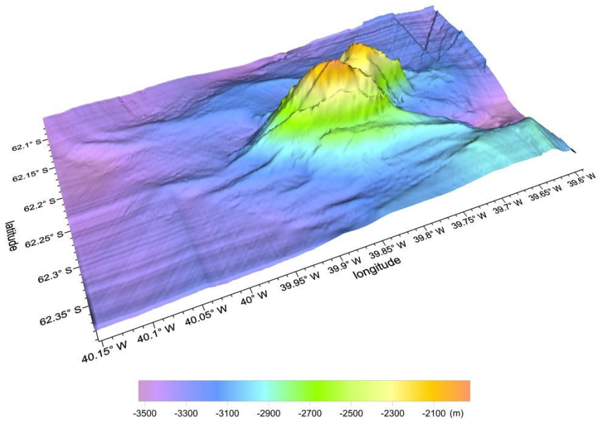
Fig.4. 3-D bathymetric map of Ziyou Hill
