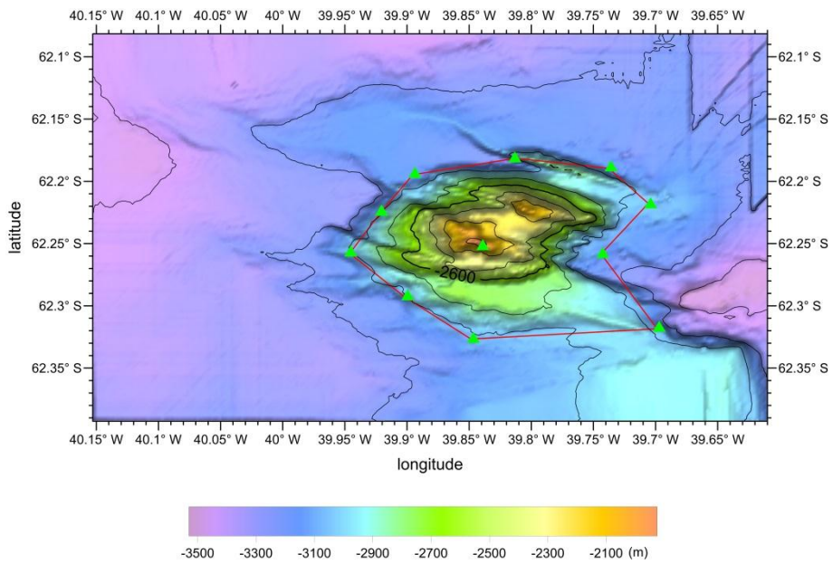
Fig.2. Bathymetric map of Ziyou Hill. Contours are in 200m
