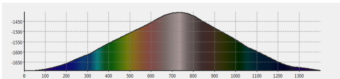
Fig.5. Profiles bathymetric map of Boniu Hill
