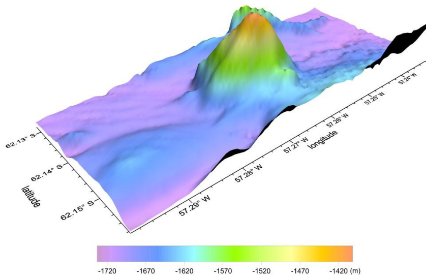
Fig.4. 3-D bathymetric map of Boniu Hill
