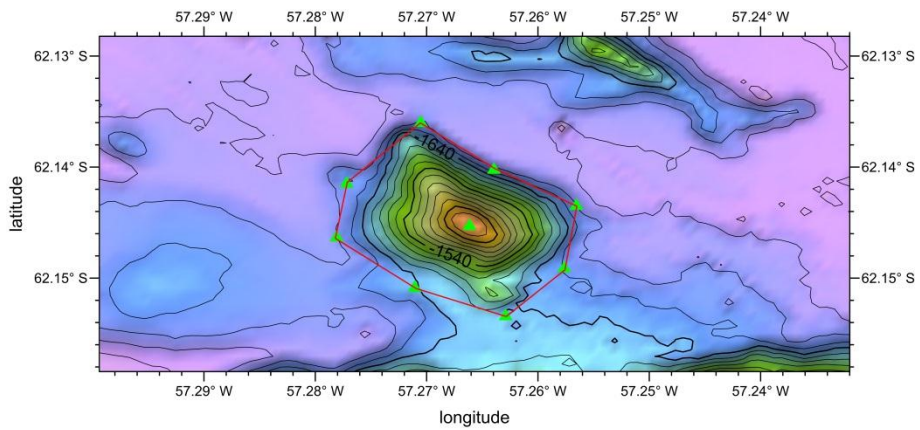
Fig.1. Index map showing the location of Boniu Hill
