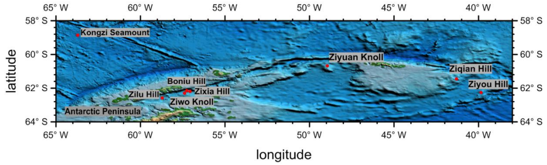
Fig.1. Index map showing the location of Boniu Hill
