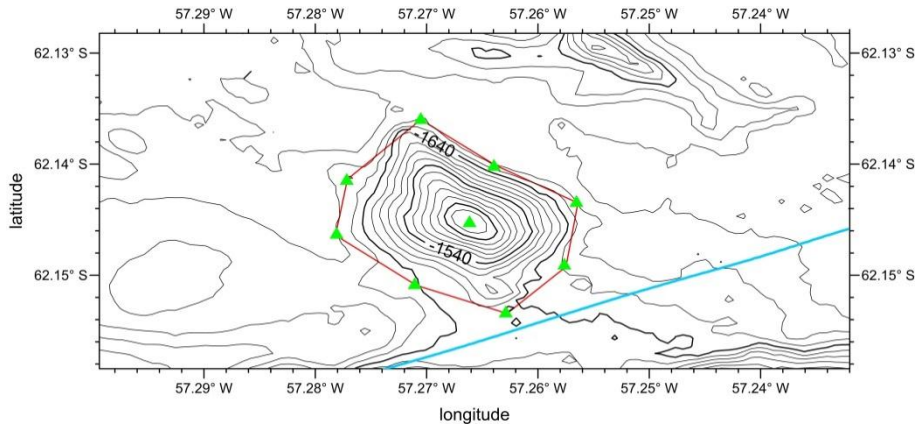
Fig.3. Bathymetric map of Boniu Hill, showing track lines. Contours are in 20m
