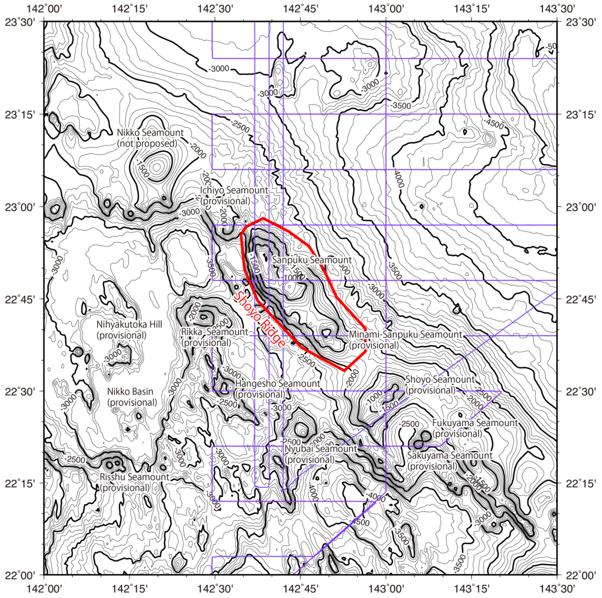
Fig. 2. Bathymetric map of the Shoyo Ridge, shown with track lines. Contours are in 100 m.
