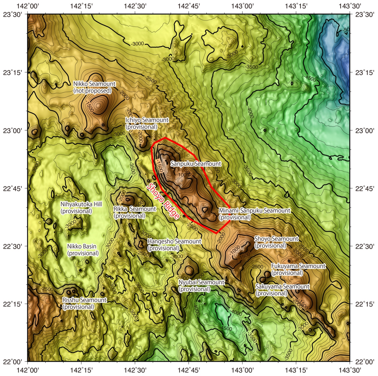
Fig. 1. Bathymetric map of the Shoyo Ridge. Contours are in 100 m.
