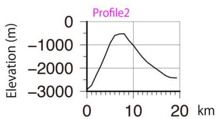
Fig. 3. Bathymetric profile across the Shoyo Ridge.
