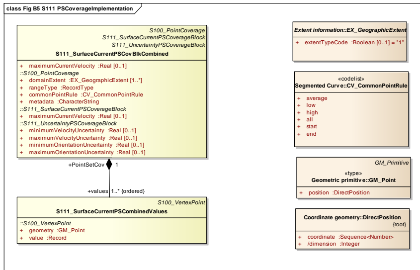
Figure B-5 - S111 Point Set Coverage Implementation
