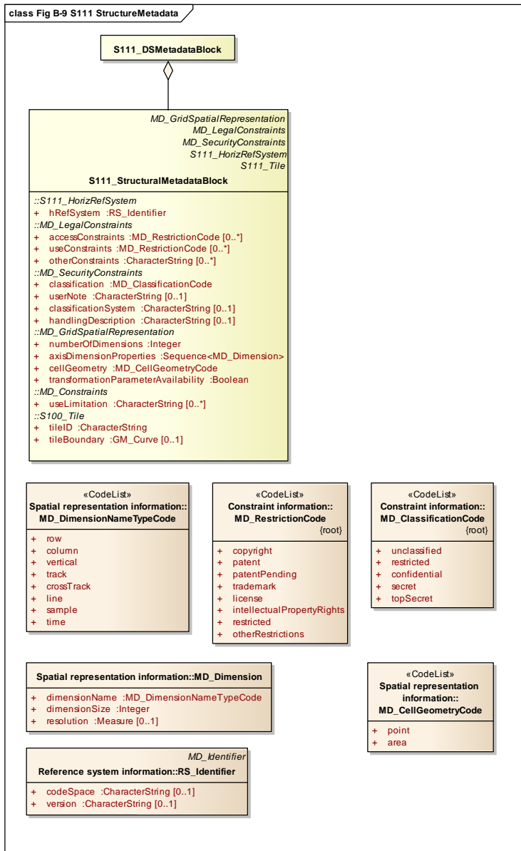
Figure B-9 - S111 Structural Metadata
