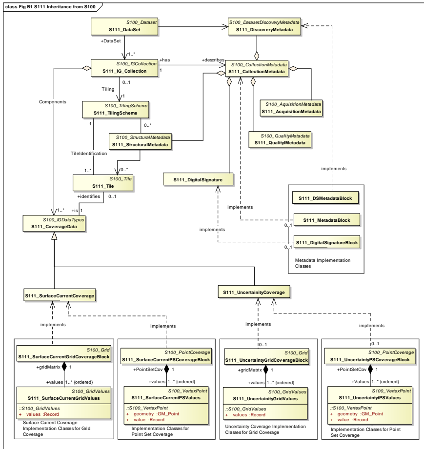
Figure B1 S-111 Inheritance from S-100
