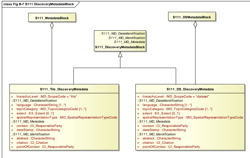
Figure B-7 - S-111 Discovery Metadata Block
