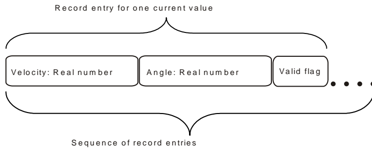
Figure 4 - Encoding Null Values in the Data Record
