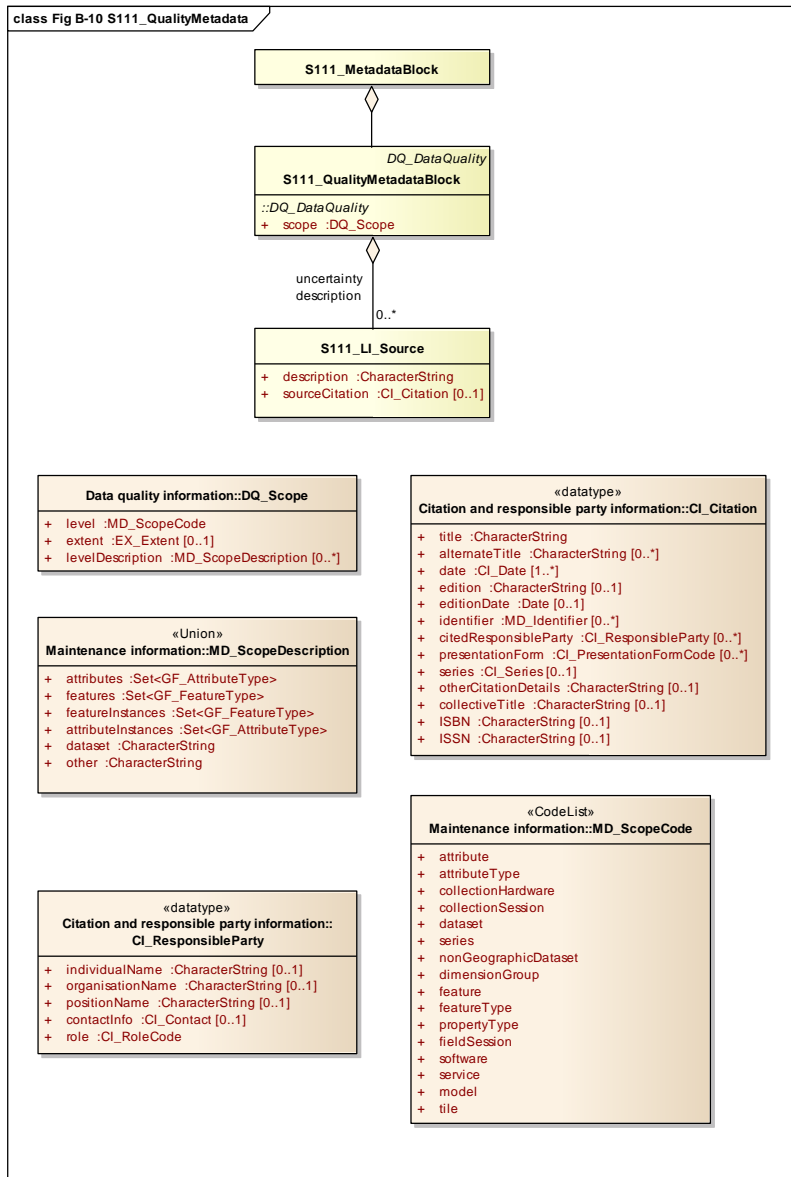
Figure B-10 - S-111 Quality Metadata Component
