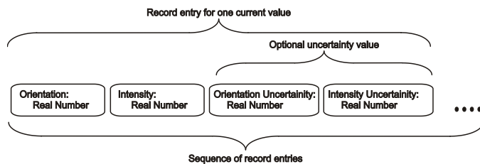
Figure B4 - S111 Surface Current Grid Coverage Record Structure with the optional uncertainty value(s).
