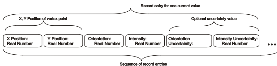
Figure B-6 - S-111 Surface Current Point Set Coverage Record Structure with the optional uncertainty value(s).
