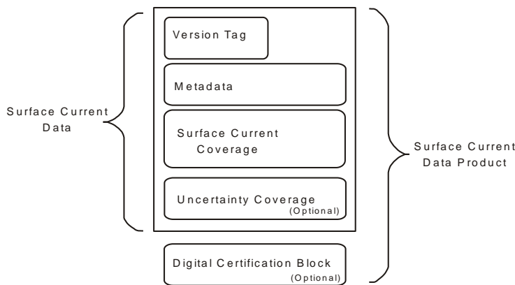
Figure 3 - Overview of Structure of Surface Current Data Product Surface Current Product
