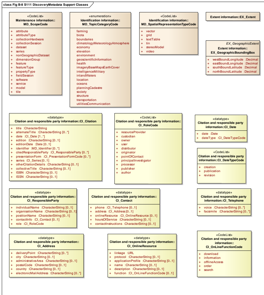
Figure B-8 - S-111 Discovery Metadata Support Classes
