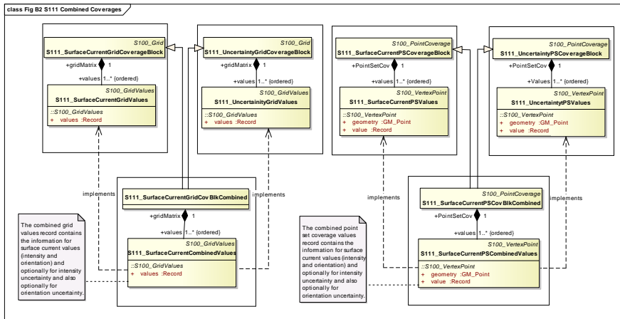
Figure B2 - S-111 Combined coverage values
