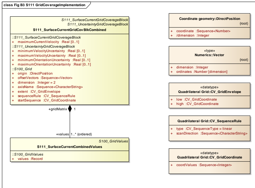
Figure B3 - S-111 Grid Coverage Implementation
