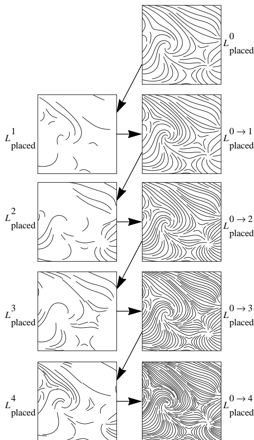
Figure 1: The process of generating multiresolution streamline-based images.
