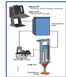
Naval Sonars
